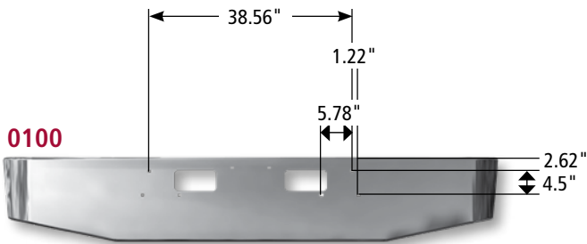
Ford L-Series conventional fits LN-LT-LTN 800, 900, 8000 and 9000 (Tow holes only). Fits trucks with 6V92 Detroit engine or 300 Cummins engine 1988 or newer (Axle forward only).
