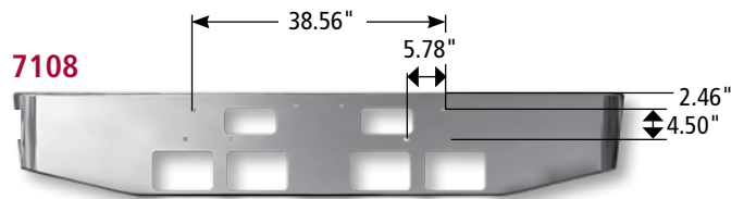
Ford Conventional LTL 9000 — Tow holes and four square light holes.
