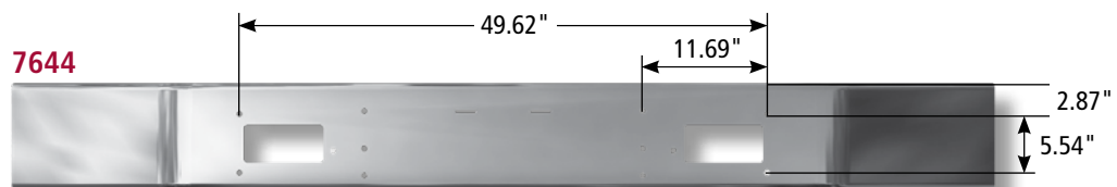
SET BACK AXLE WITH TOW HOLES AND COW CATCHER HOLES
